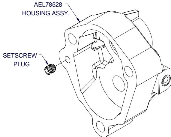
Figure 1: AEL78531-1 Assembly
